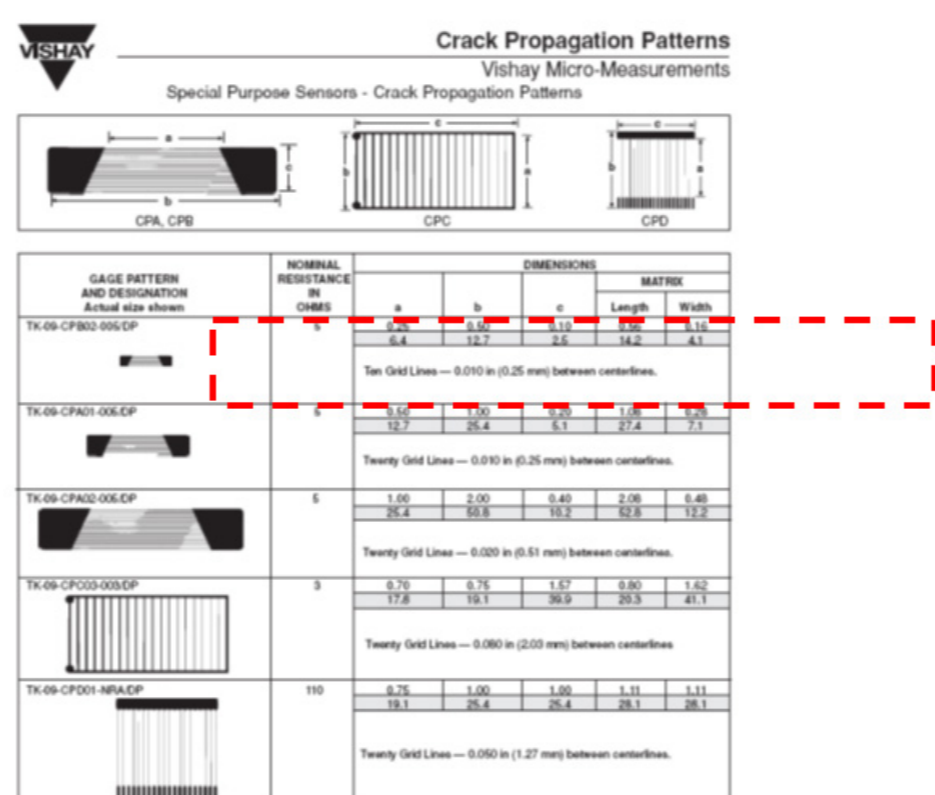
Figure 5: Datasheet of Vishay crack propagation gages 10.
